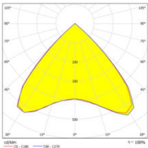
BO198-Glitter-2x2-5050-90°(Sq.-Beam)
