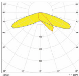
BO107-Custom-9x1-5050-Type-IIS
