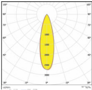
BO174-Sunbeam-1x1-5050-RGBW-25°
