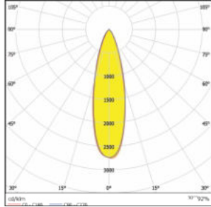
BO175-Sunbeam-1x1-5050-25°(Gen1)
