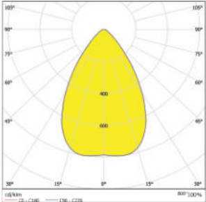
BO10-Shimmer-16x1-2835/3030-60°
