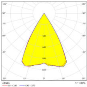
BO198-Glitter-2x2-5050-60°(Sq.-Beam)
