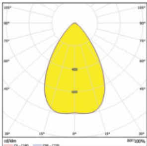
BO204-Custom-20x1-5050-60°
