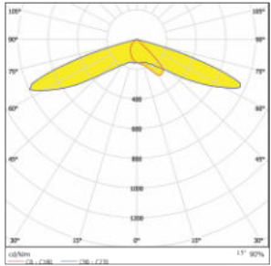
BO42-Sunbeam-1x1-3535-70x140°
