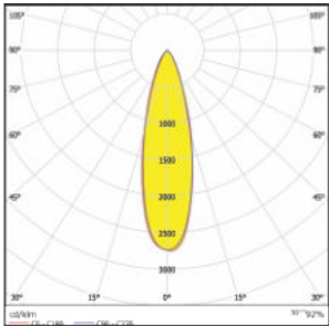
BO176-Sunbeam-1x1-5050-25°(Gen2)
