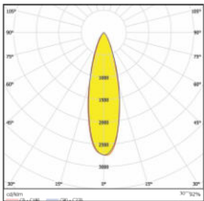
BO23-Shimmer-16x1-2835/3030-20°
