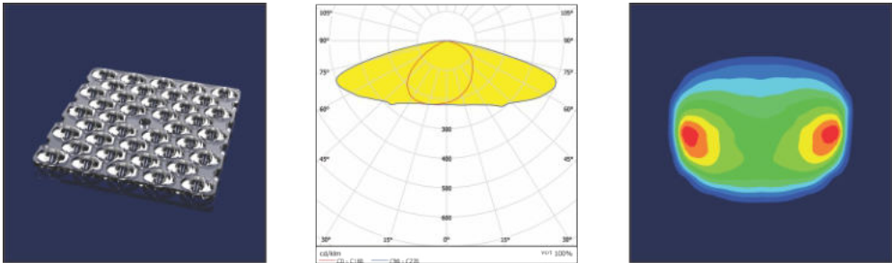
BO54-Oculus-40x1-2835/3030-Type-II
